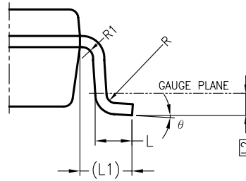
VIEW B
